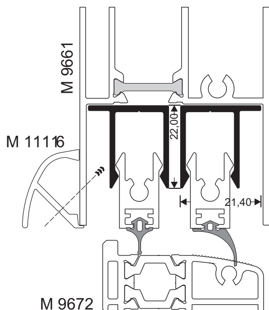
PROFIL ZA DNO VRATA SUPPLEMENTARY PROFILE FOR DOORS M 11211 W=268 gr/m
