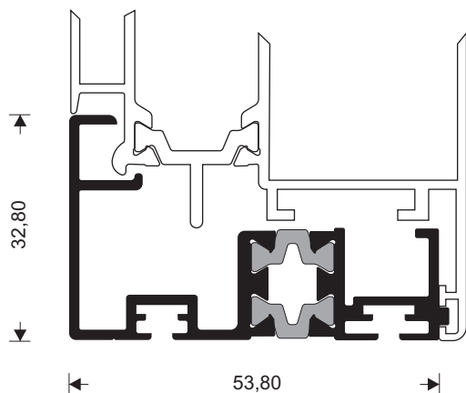
DODATAK ZA DNO VRATA SUPPLEMENTARY PROFILE FOR DOORS M 9681 W=890 gr/m
