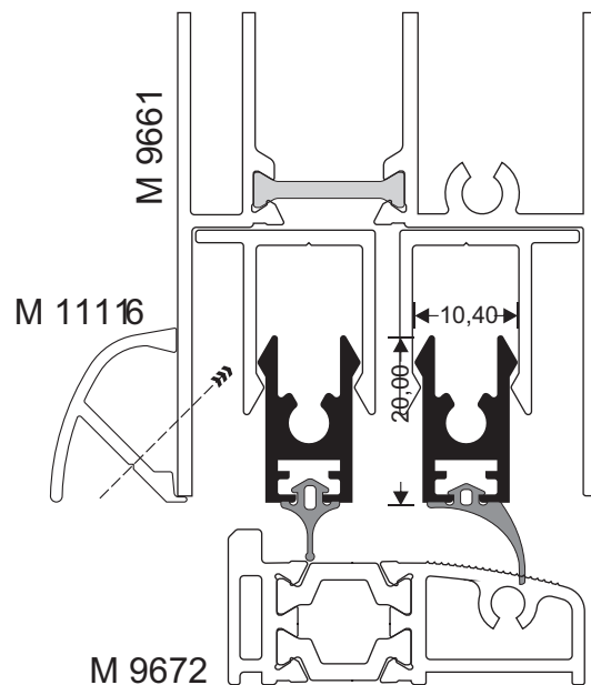
PROFIL ZA DNO VRATA NOSAČ GUME SUPPLEMENTARY PROFILE FOR DOORS M 11210 W=283 gr/m
